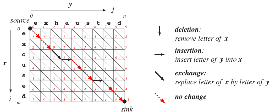
Figure 8.9: The edit distance calculation for strings \mathbf{x} and \mathbf{y} can be illustrated in a table. Algorithm 3 begins at source , i = 0, j = 0 , and fills in the cost matrix \mathbf{C} , column by column (shown in red), until the full edit distance is placed at the sink , \mathbf{C}[i = m, j = n] . The edit distance between “excused” and “exhausted” is thus 3.
